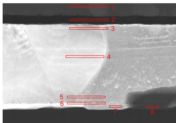
Figure 2 STEM image of Cu Metal 1 on Ohmic
