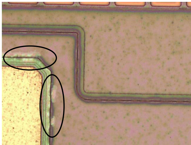
Figure 1 Exposed Cu attacked in pre-clean solution.
