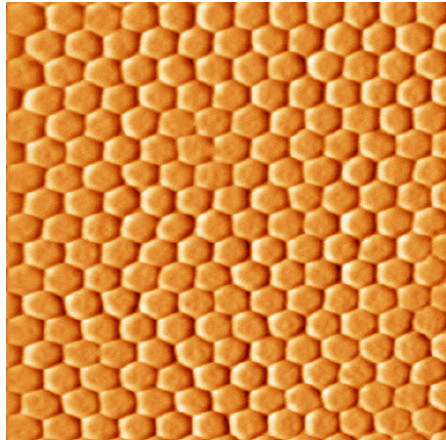
Figure 1 Micrograph of patterned InGaAs/GaAs quantum dots. Each dot is less than 100 nm wide.
