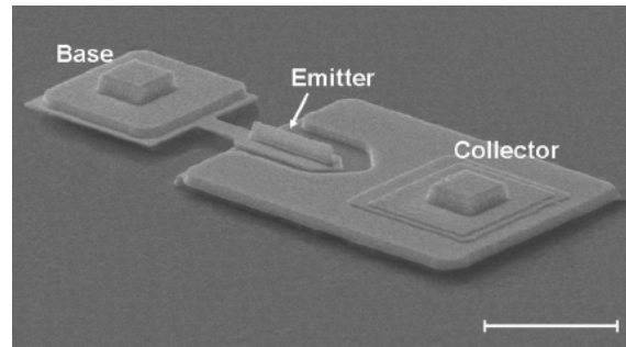
Figure 2 Micrograph of pseudomorphic InP/InGaAs HBT.
