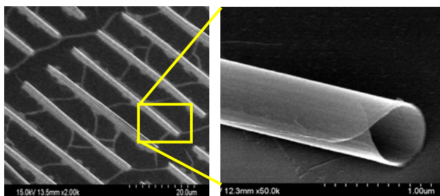
Figure 3 Self-rolled compound semiconductor nanotubes.
