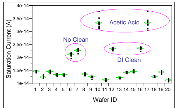
Fig 3: BC diode saturation current comparison
