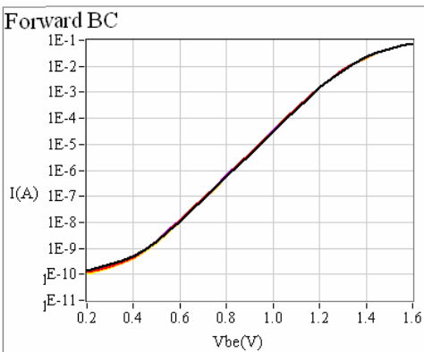
Figure 7: Stable I-V of the BC diode with lower turn on voltage over reliability stress.
