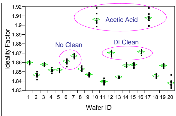
Fig 2: BC diode ideality factor comparison
