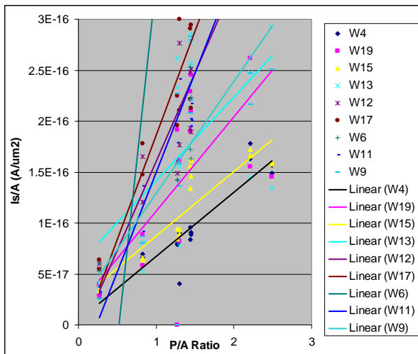
Figure 8: Plot of saturation current vs. periphery over area ratio.
