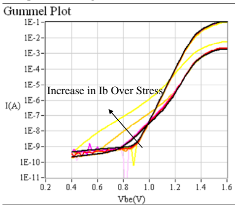
Figure 6: Gummel plots of a transistor with early wear out failure over reliability stress
