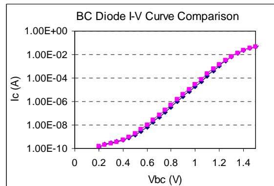
Figure 4: Comparison between the I-V curves of a good diode and an abnormal diode. The purple one is measured from the wafer processed with no clean and the blue one is from the wafer with \text{NH}_4\text{OH} cleaning.
