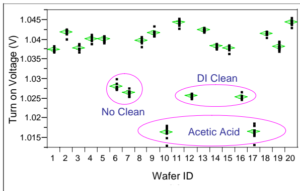
Fig 1: BC diode turn on voltage comparison
