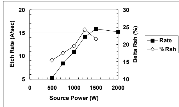
Figure 2. Etch rate and increase in Rsh as a function of source power at 10mTorr. RF bias power was left constant at 5W.
