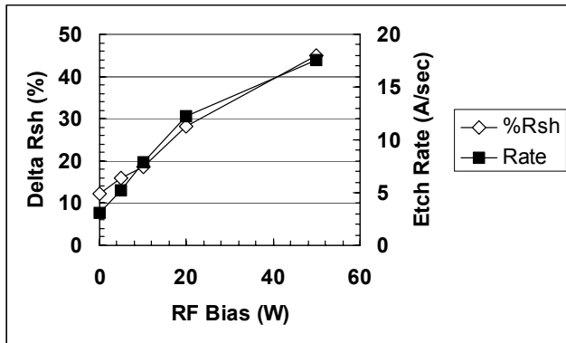
Figure 1. Etch rate and increase in Rsh as a function of RF bias power at 10mTorr. Source power was left constant at 500W.
