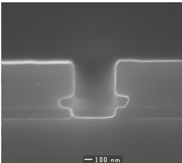
Figure 5. SEM cross-section of a representative gate profile after completion of the low damage etch. The undercut is part of the photolithography process.
