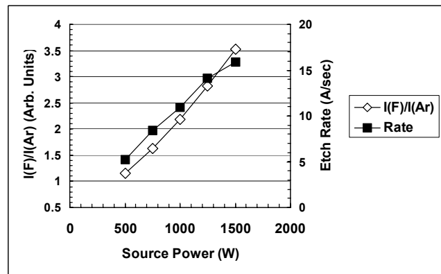
Figure 3. Etch rate and relative fluorine concentration at a pressure of 10mTorr and 5W RF bias power.
