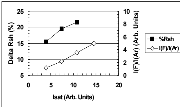
Figure 4. Effect of ion saturation current on induced semiconductor damage Rsh.
