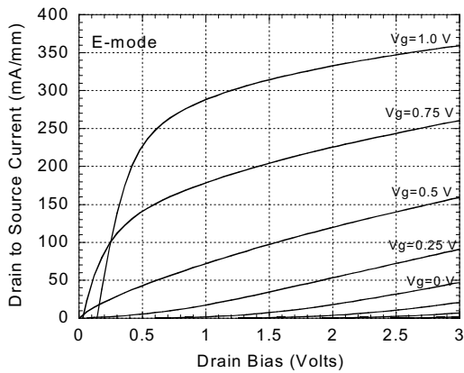
Fig. 3 D-mode and e-mode I-V curves
