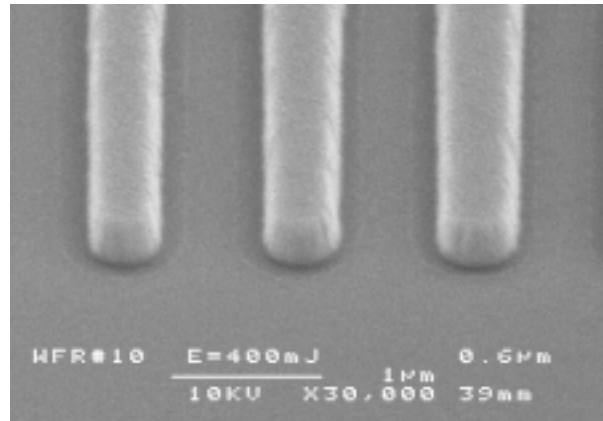
Figure 4. Equal line-space 0.6μ metal lines following lift-off.
