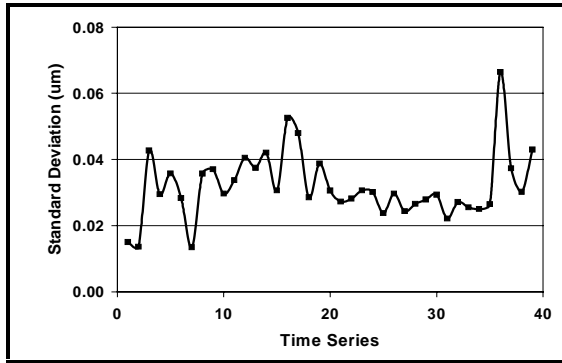
Figure 5. Standard deviation of 1.2 \mu nominal photo feature for 150 mm wafers (Apr to Nov. 2000)
