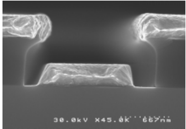
Figure 3. Photoresist profile following metal evaporation.
