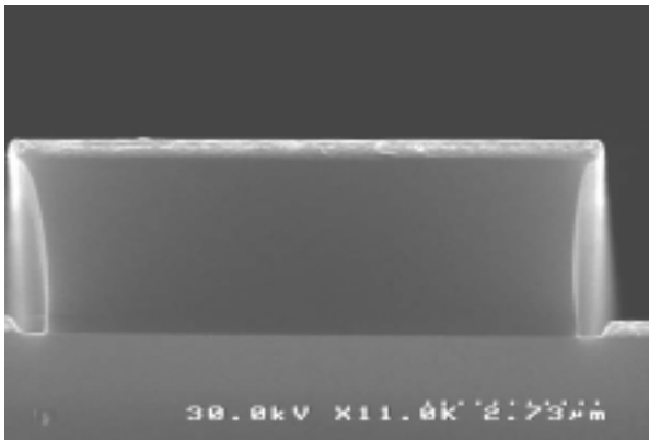
Figure 6. Photoresist profile following metal evaporation for large topography lift-off .
