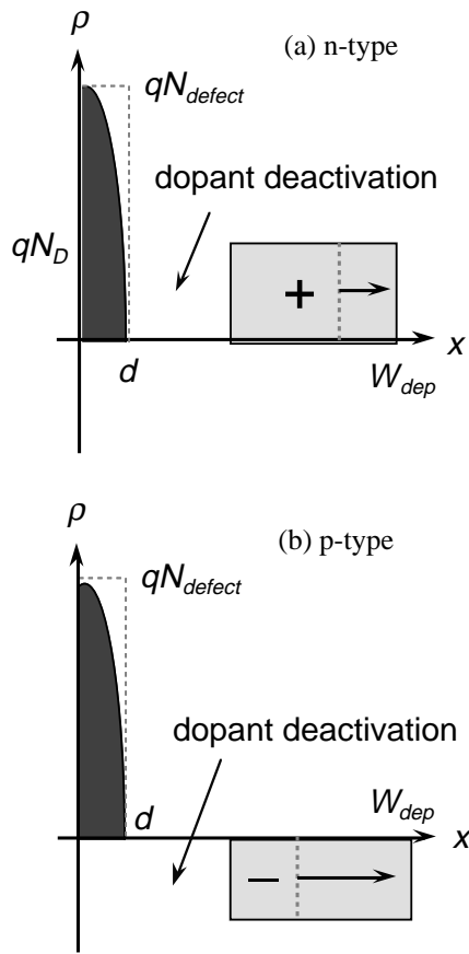
Fig. 4 A schematic illustration of the space-charge distribution in the depletion layer of the Schottky contacts formed on the hydrogenated GaAs surface. Since hydrogen deactivates both donor and acceptor, the depletion-layer width would increase. On the other hand, the near-surface defects modify the effective barrier height, which is mainly responsible for I-V characteristics.
