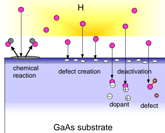
Fig. 1 Hydrogen impinges on the GaAs surface resulting in (1) surface stoichiometry change, (2) introduction of near-surface defects and (3) deactivation of dopants and bulk defects.
