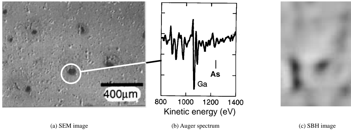
Fig. 2 Reductive reaction of native oxides with atomic hydrogen changes the surface stoichiometry of GaAs, resulting in formation of Ga droplets at low temperatures. The Schottky contacts formed on such a surface become inhomogeneous.
