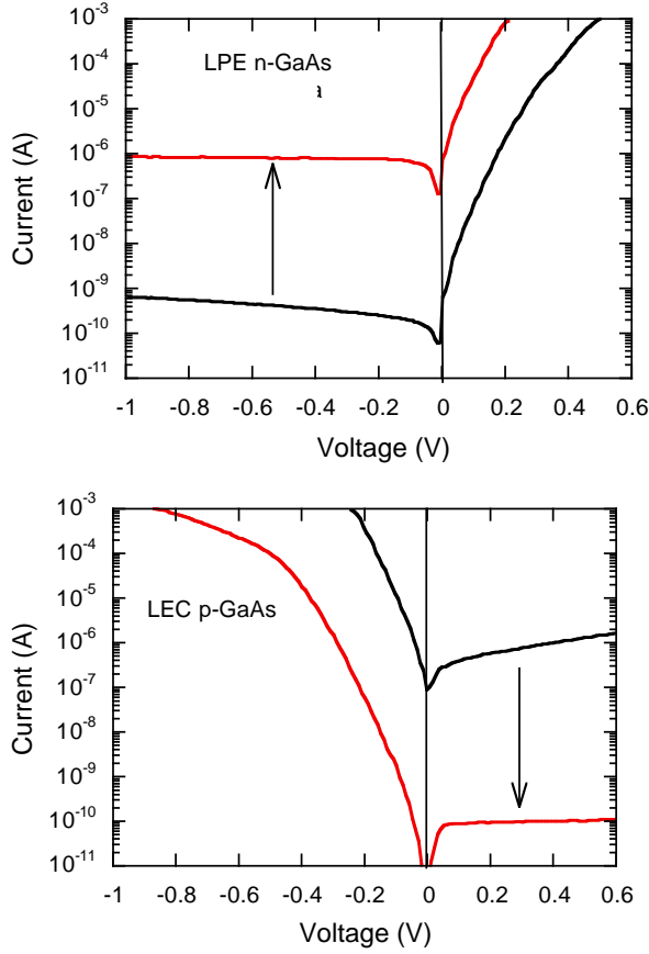
Fig. 3 Upon hydrogenation of the GaAs surface, the apparent SBH becomes low and high for n- and p-type substrates, respectively. The near-surface defects acting as a donor are responsible for the effective change in SBHs.
